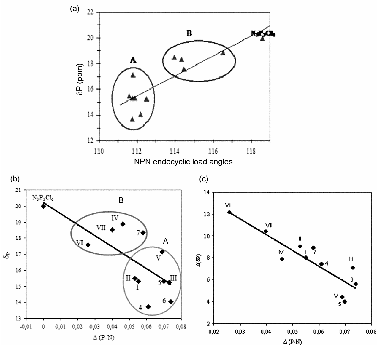
Figure 5. The relationships between (a) \delta P_{(\text{spiro})} -values and endocyclic NPN ( \alpha ) angles. (b) \delta P_{(\text{spiro})} -values and \Delta(P-N) . (c) \Delta(\delta P) values and \Delta(P-N) . \delta(PCl_2) and the \alpha -values of N_3P_3Cl_6 are 19.60 ppm, 118.30(2)°. 32 Region A indicates monotopic tetrachloro-phosphazenes, Region B indicates pyrrolidiny-substituted and ditopic spiro -crypta phosphazenes.
